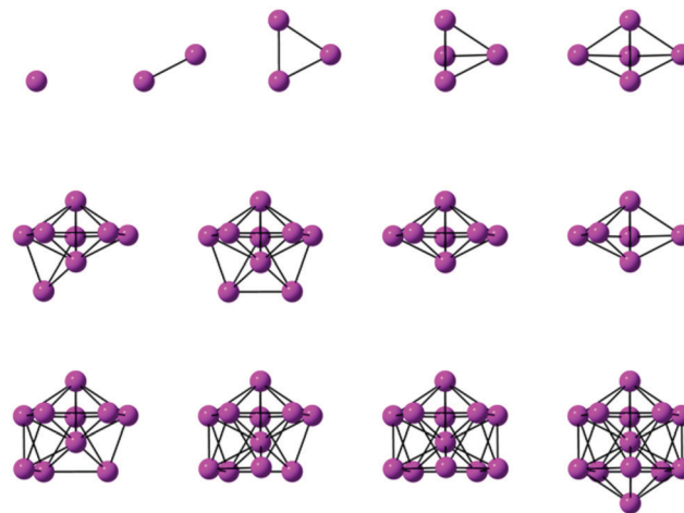
Fig. 1 Illustration of icosahedral \text{Ag}_{13} cluster formation from a single Ag atom.
